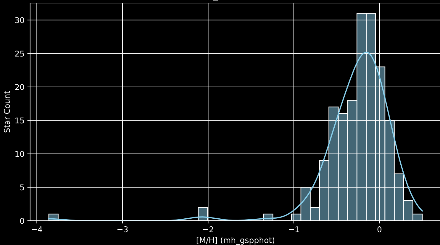
APOGEE DR17 Field: [199+46_MGA [M/H] (mh_gspphot) (n= 183)
