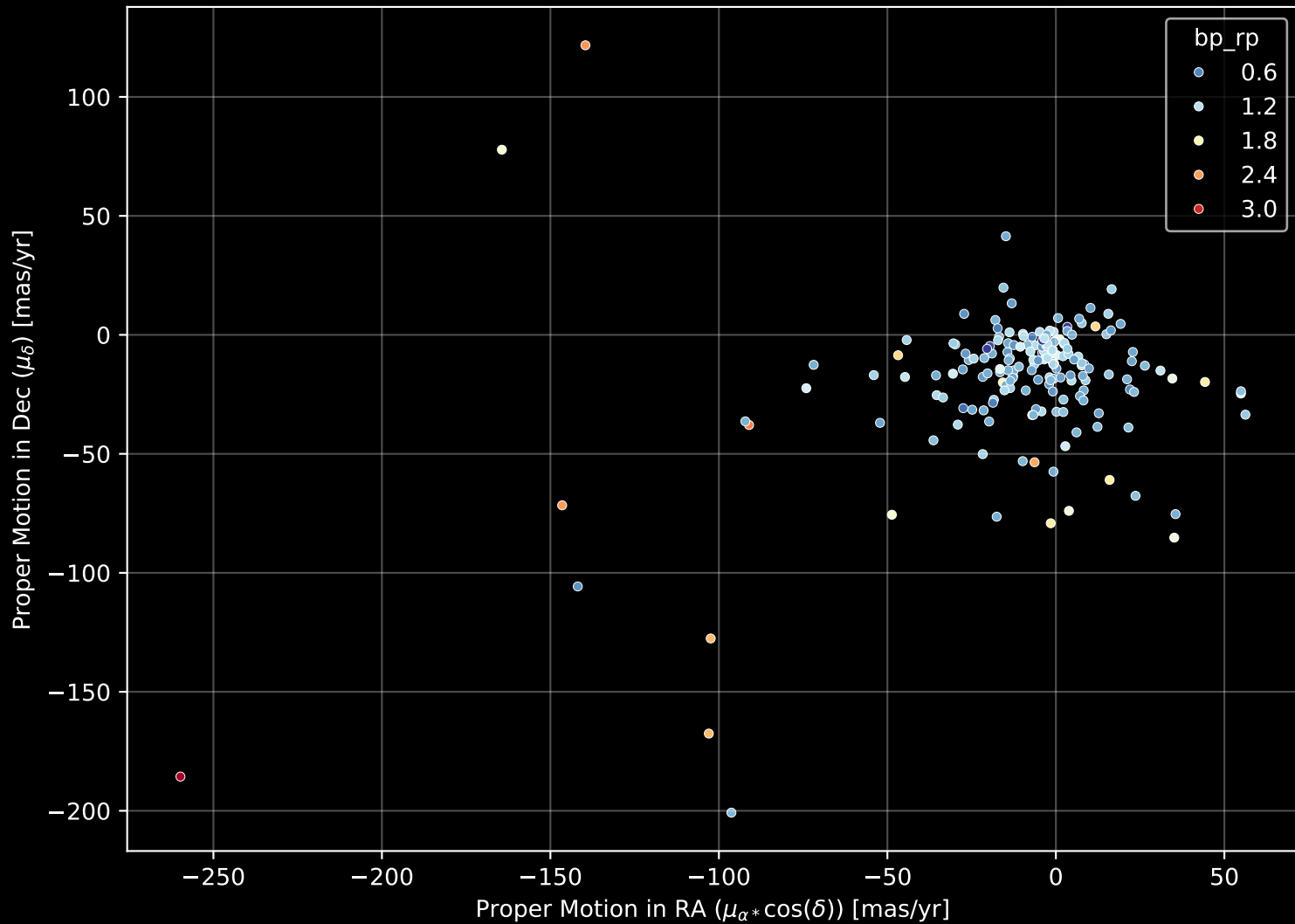
APOGEE DR17 Field: [199+46_MGA] Proper Motion Diagram (n= 185)
