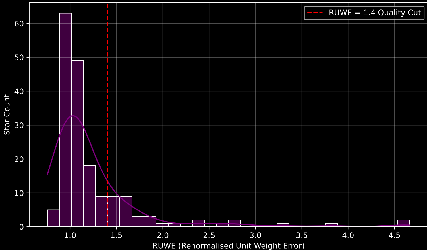
GAPOGEE DR17 Field [199+46_MGA] RUWE Distribution (n= 179)
