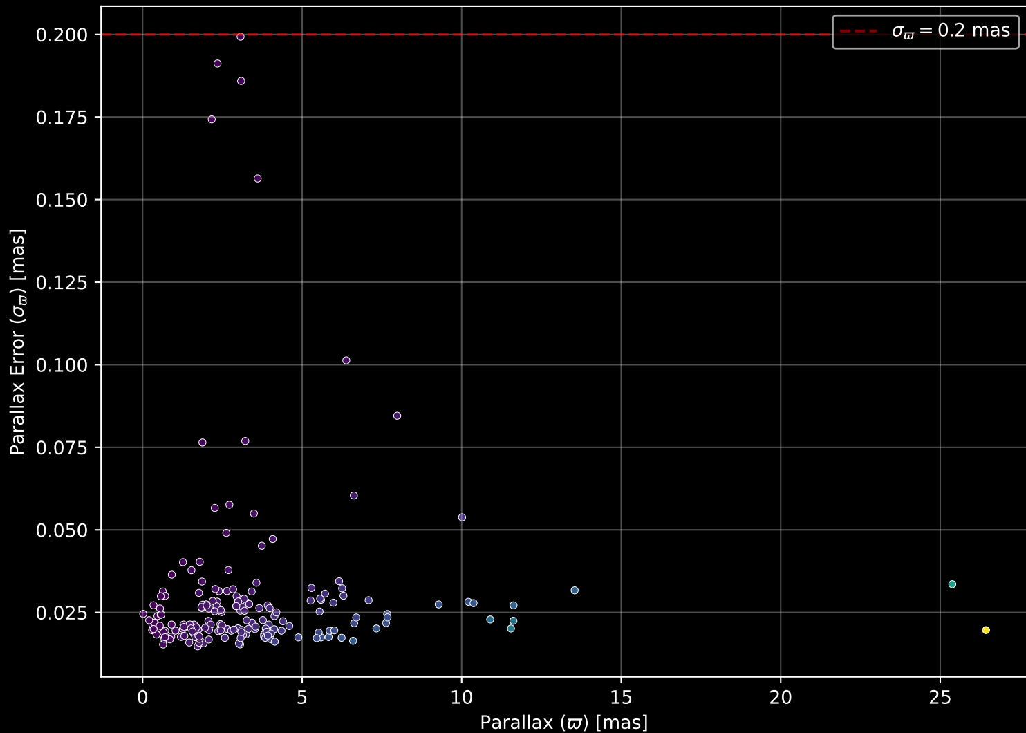
APOGEE DR17 Field: [199+46_MGA] Parallax Quality (n= 185)
