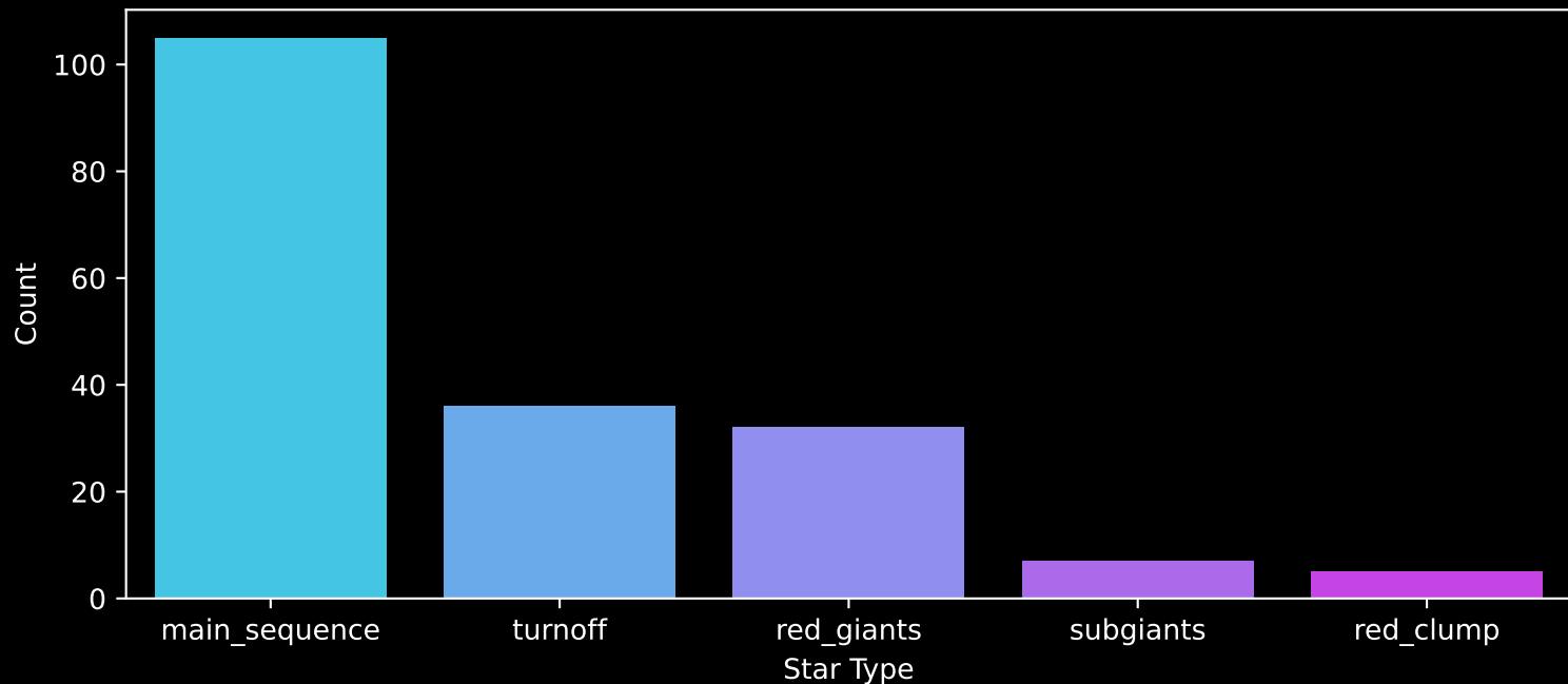
APOGEE DR17 Field: [199+46_MGA] Count plot of Star Type
