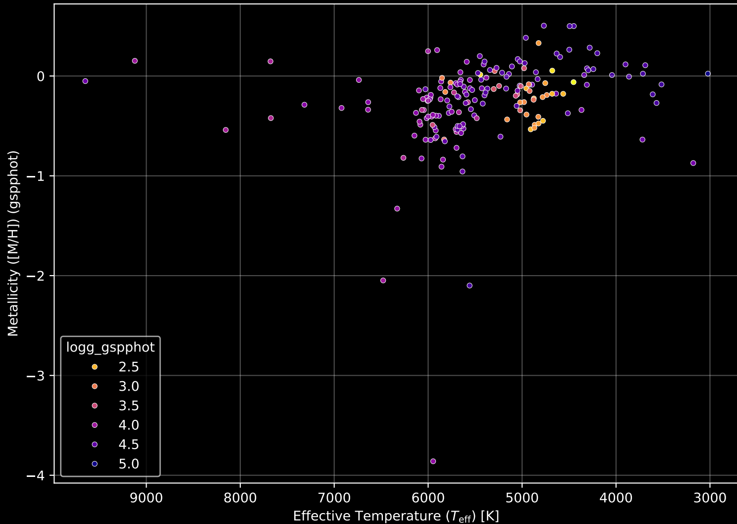
APOGEE DR17 Field: [199+46_MGA] Stellar Population Parameters (n= 185)
